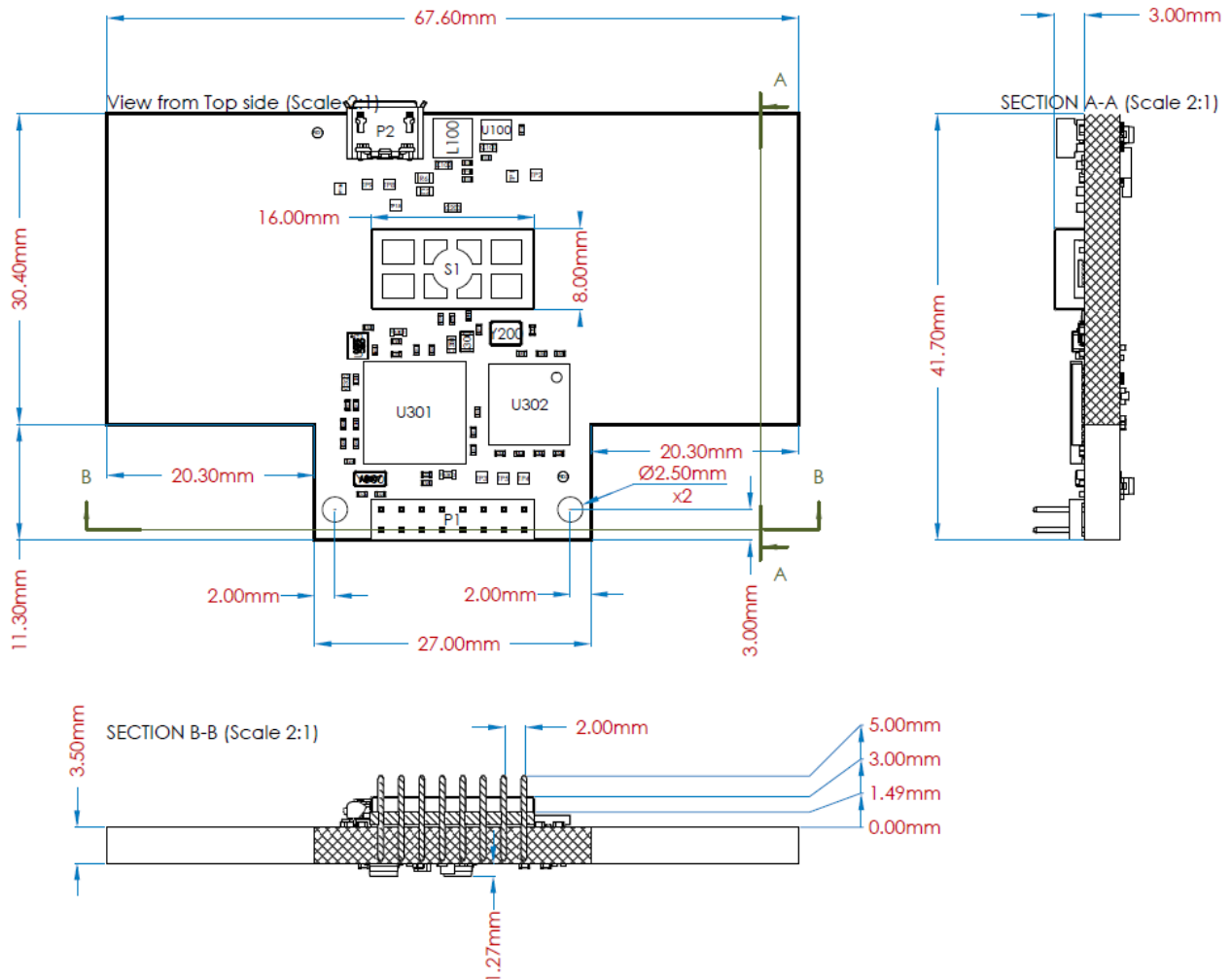
Mechanical drawing of the sensor module (in mm)
