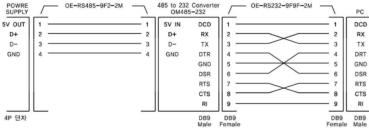
485 to 232 Converter
